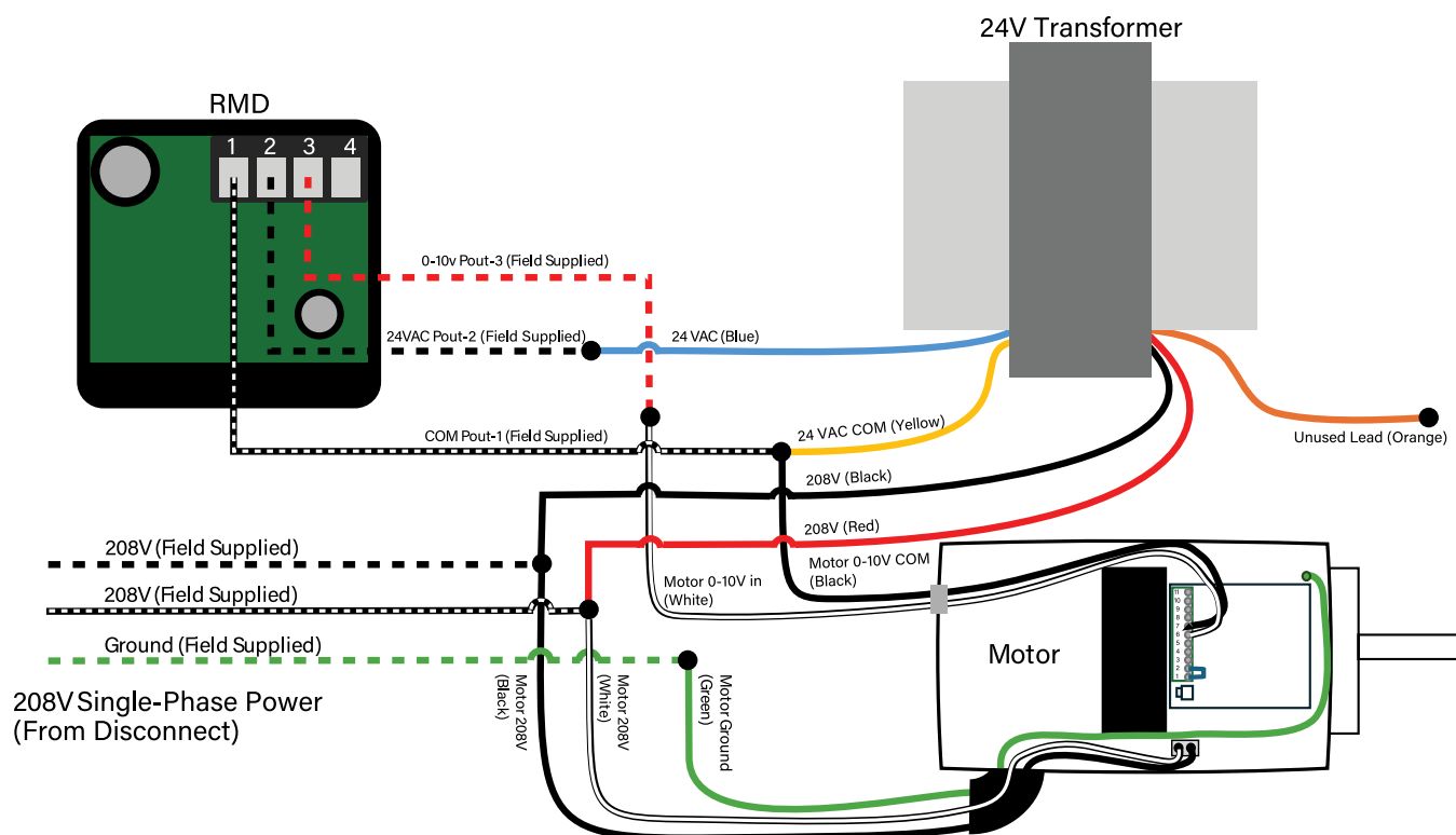
ABB EC Titanium 208V RMD Wiring Schematic
