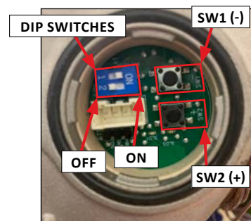
Remote Mounted Dial
