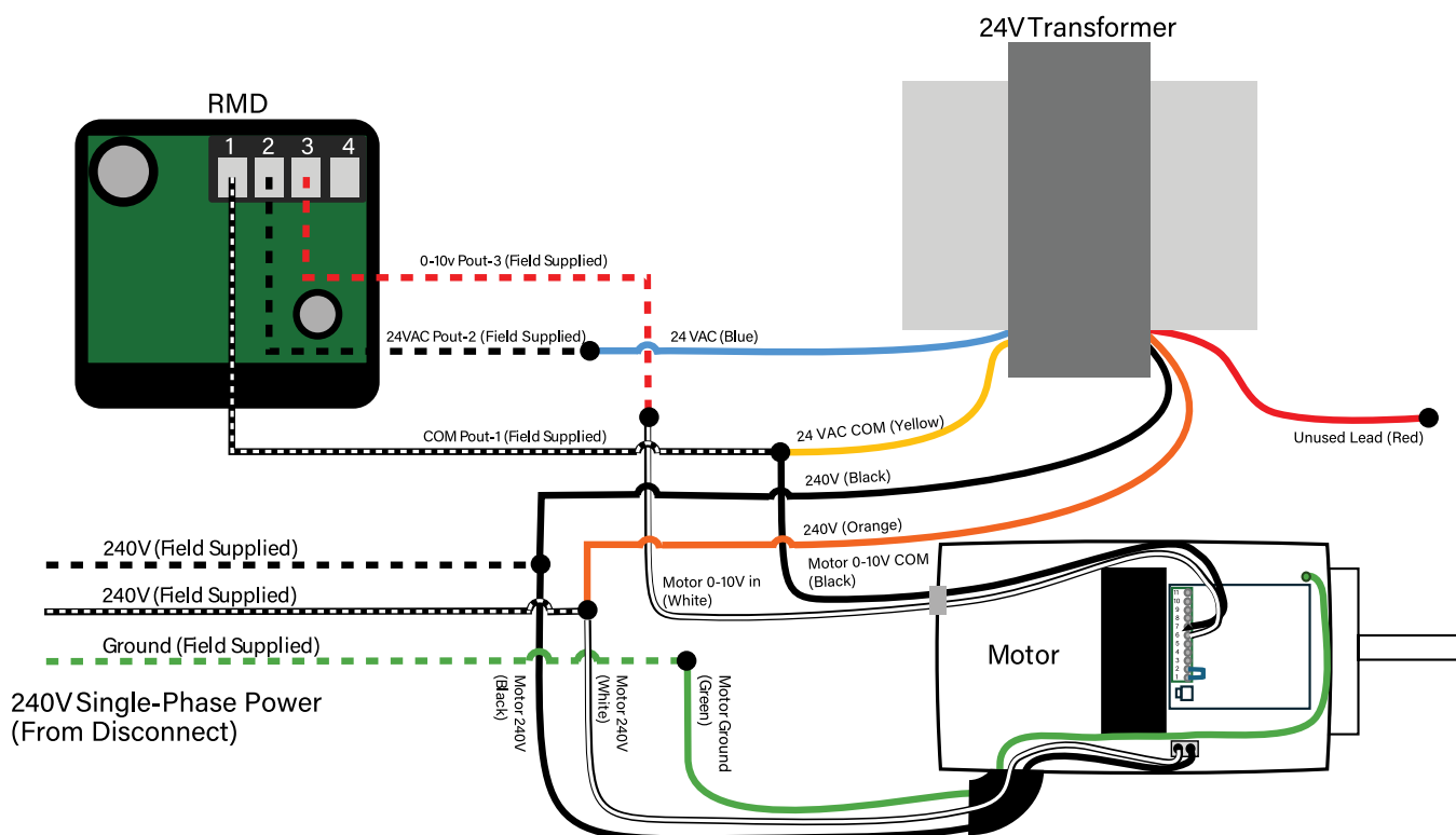
ABB EC Titanium 240V RMD Wiring Schematic
