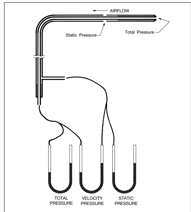
Figure 1. Pitot Tube
