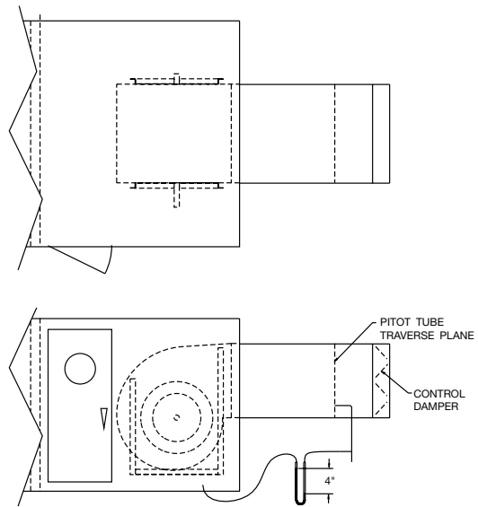
Figure 20. Air Handling Unit With Added Duct
