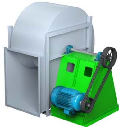
Arrangement 9
