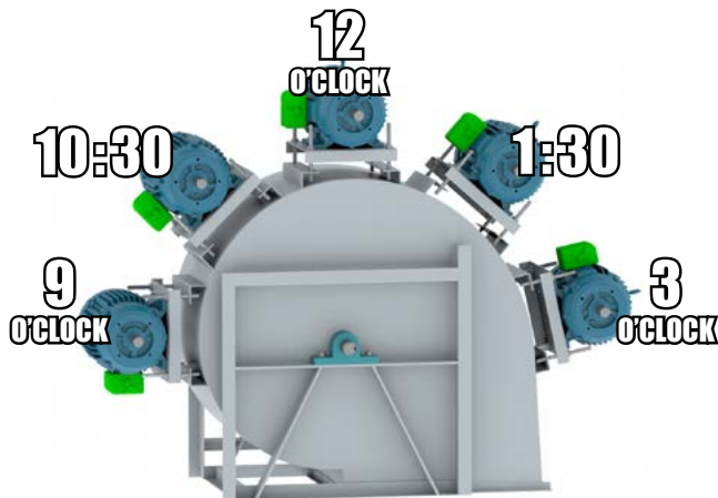
DBD Discharge
