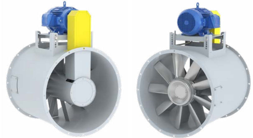
Arrangement 9 Belt Driven
