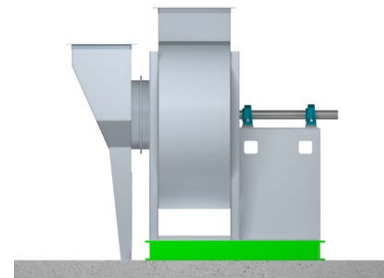
FAN MOUNTED ON UNITARY BASE AND INLET BOX MOUNTED ON GRADE (LEGS TO GRADE)
