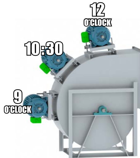
THD Discharge
