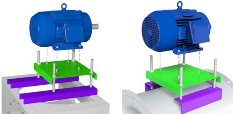
Flat Mount
