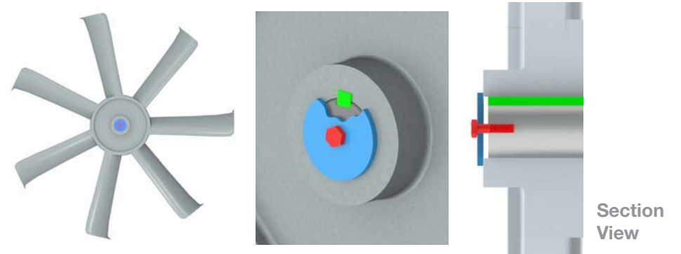
STRAIGHT BORE HUB (WITH KEY, RETAINING WASHER AND BOLT)
