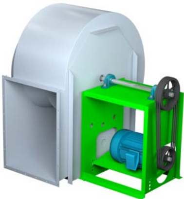
Arrangement 10
