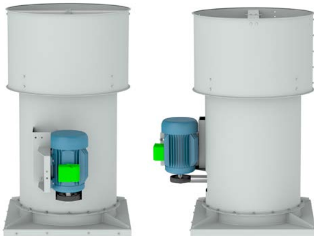
Roof Mounted
