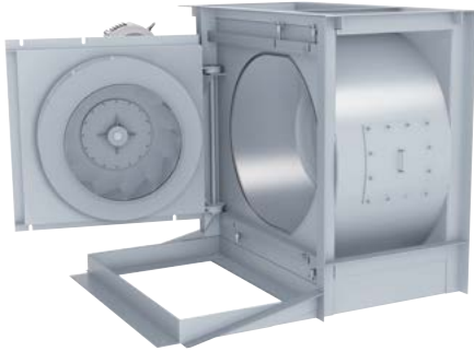
Centrifugal Swingout Fans
