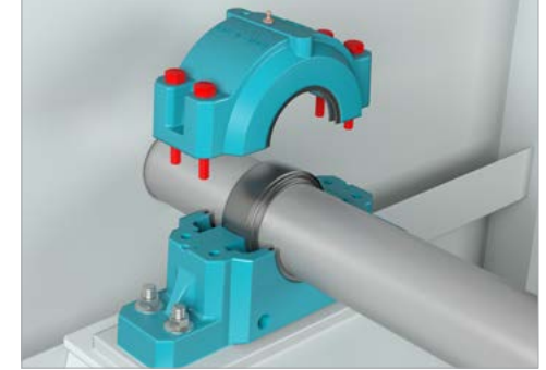
SPLIT PILLOW BLOCK BEARING ROLLING ELEMENT: OFFERED IN BALL TYPE AND SPHERICAL ROLLER TYPE
