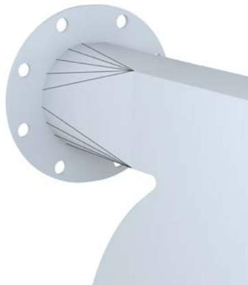
Welded Rectangular/ Square to Round Transition with Outlet Flange
