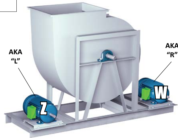
Arrangement 3F
