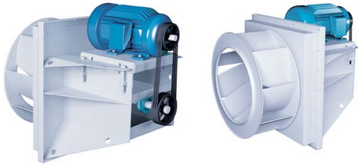
Arrangement 9 Belt Driven Fan is wall mounted
