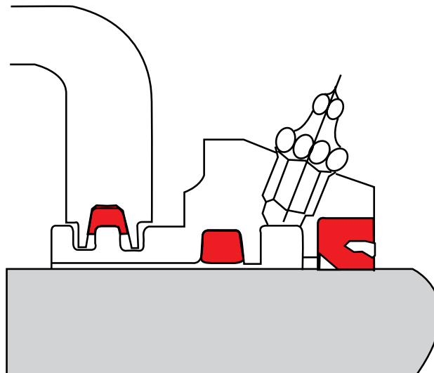
Taconite Seal
