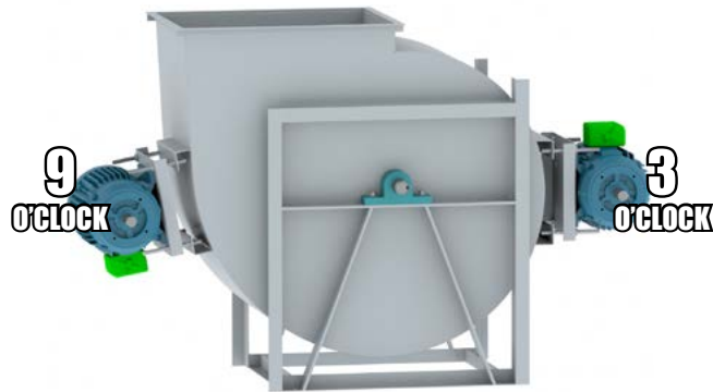
UBD Discharge
