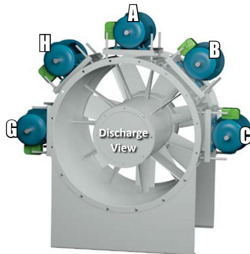
Floor Mount
