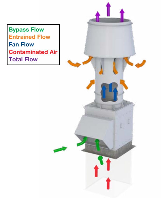
TUBULAR INLINE CENTRIFUGAL & MIXED FLOW LAB EXHAUST FAN
