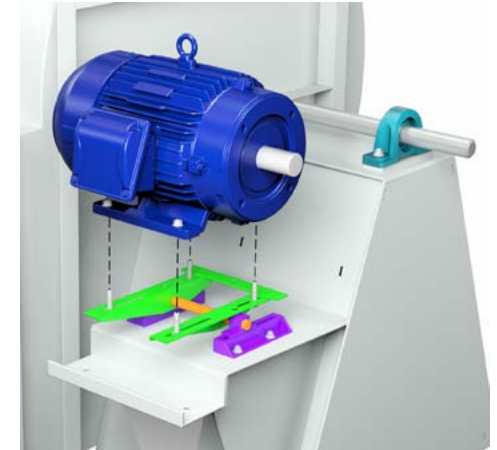
Arrangement 9H Centrifugal Fan
