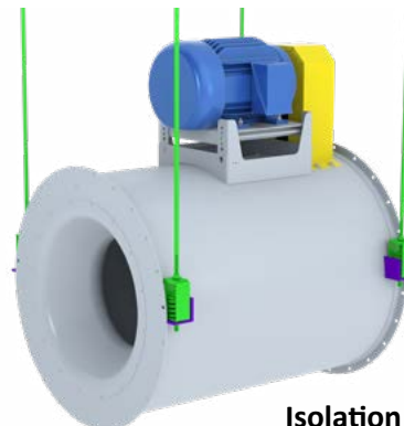
Isolation Hangers
