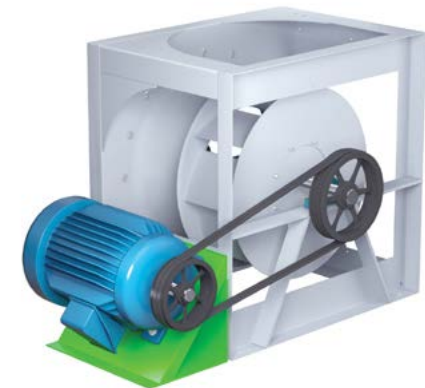
Arrangement 3SM
