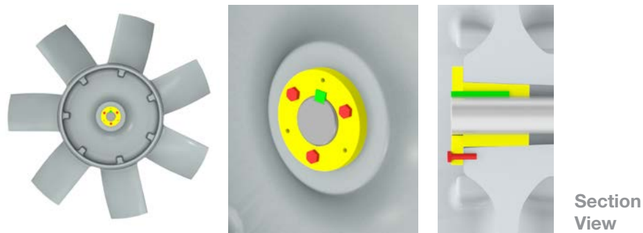
TAPER LOCK HUB/BUSHING (WITH KEY AND HARDWARE)
