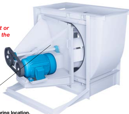
Arrangement 9SS Belt Driven - S wingout Construction Pivot Base S ide Mounted Motor
