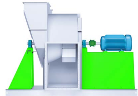
Arrangement 7SI
