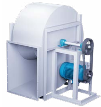
Sizes 402+ (Vent Sets) Motor Mounted on Slide Base on Side of Pedestal
