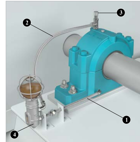
STATIC OIL LUBRICATION SYSTEM (TRICO OILER)
