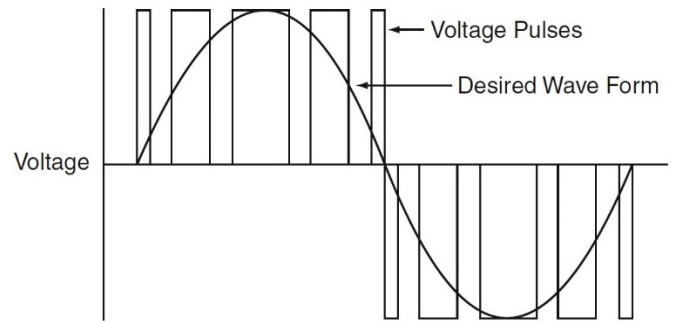
Figure 2: Single-Phase, Three-Level PWM waveform.
