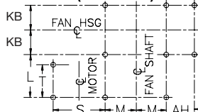
TEN 'BH' DIA. BASE HOLES FOUNDATION PLAN
